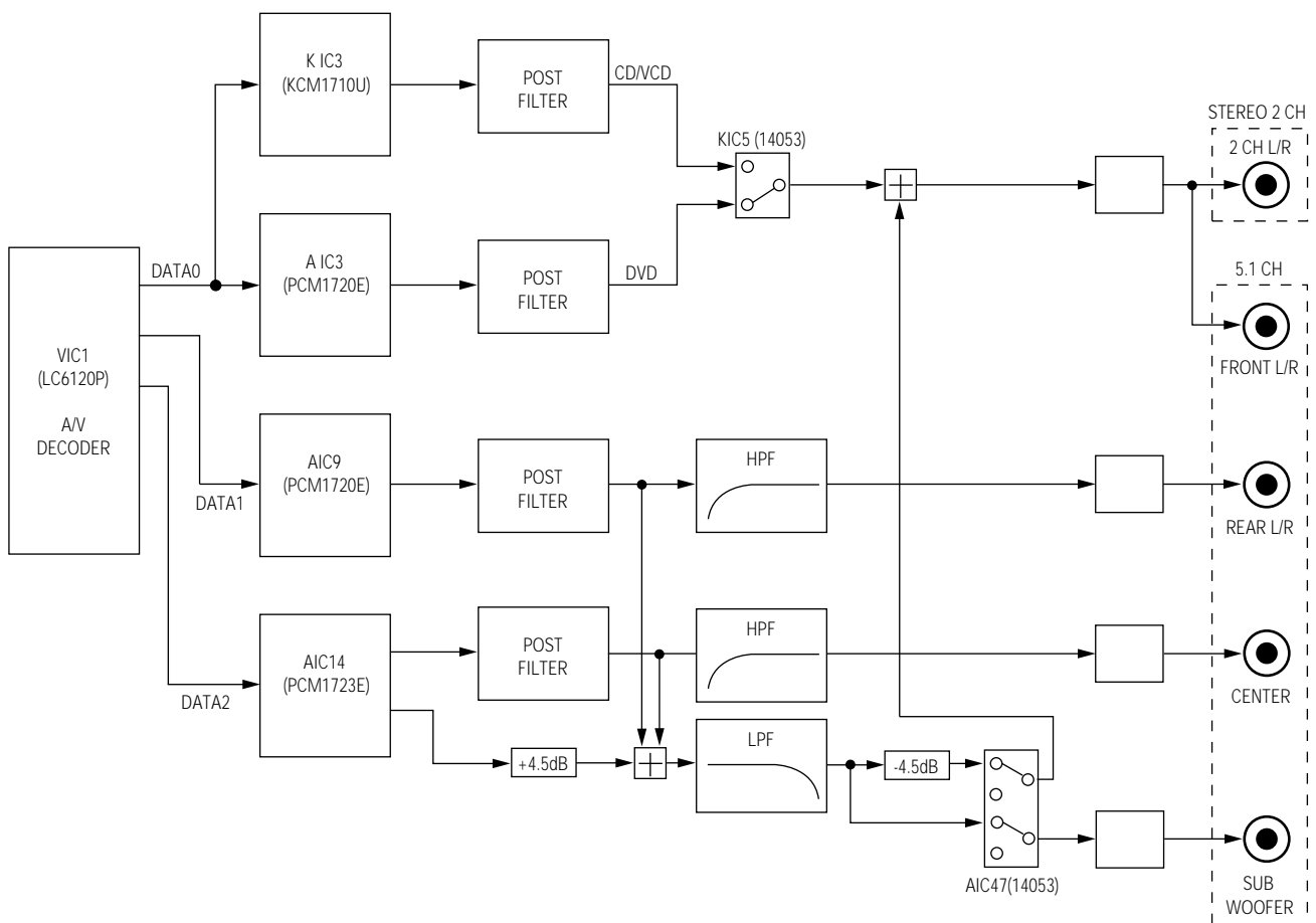
Fig. 2-55 Audio output block diagram
