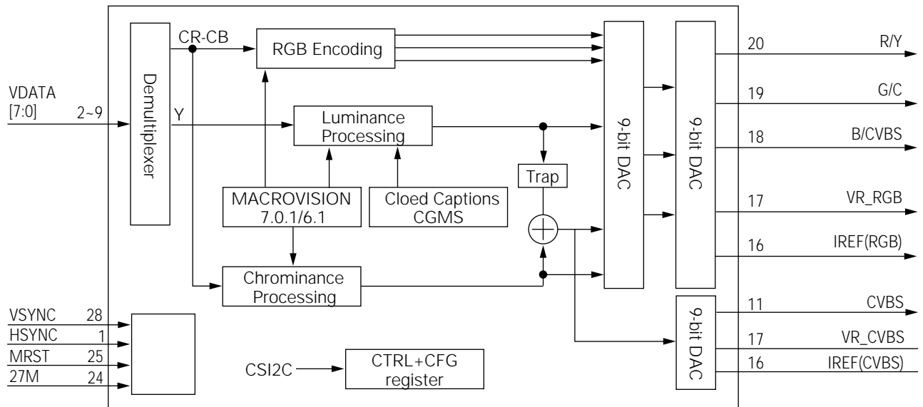
Fig. 2-51 VIC3(STV0119) internal block diagram
